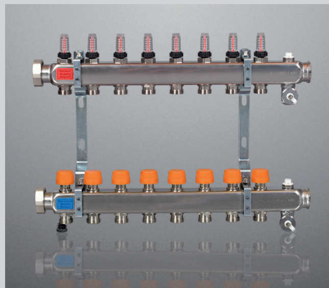
Heating circuit manifold with flow meter
